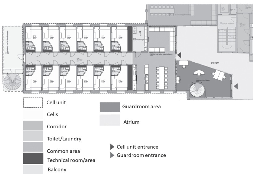
Figure 2. Illustration of a wing second/third floor and central component
